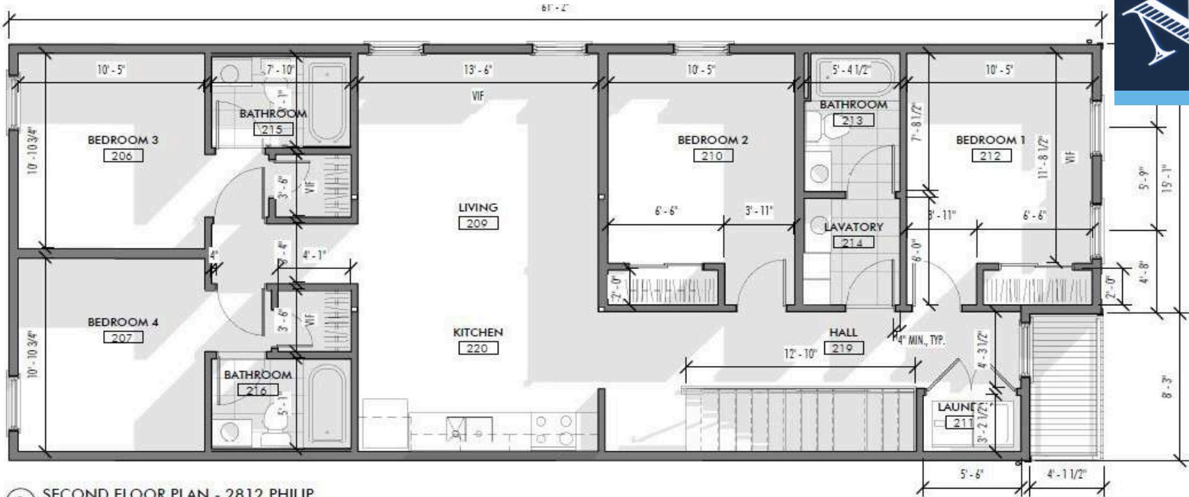
2 SECOND FLOOR PLAN - 2812 PHILIP 3/16" = 1'-0"
