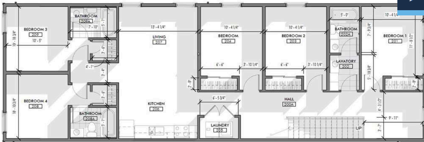
2 SECOND FLOOR PLAN - 2808 PHILIP 3/16" = 1'-0"
